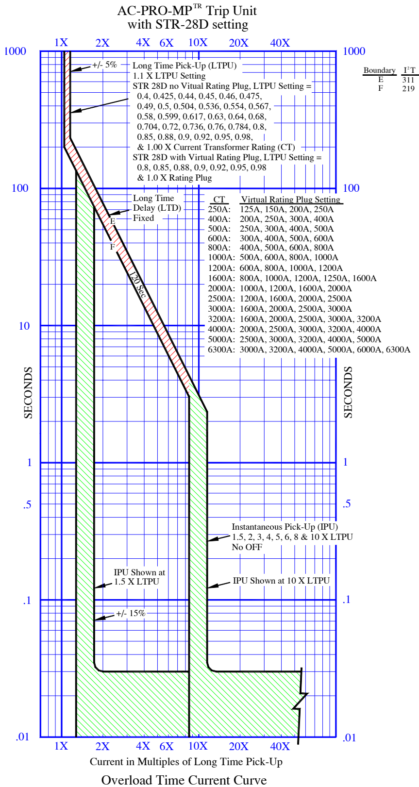
Figure 6 AC-PRO-MP TM STR-28D Time-Current-Curve
